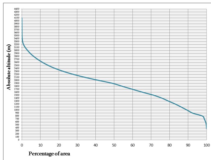
Figure 2. Percentage hypsometric curve of the territory of the Republic of Armenia.
