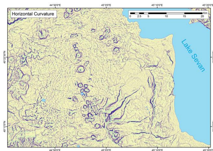
Figure 4. Volcanogenic CS on the horizontal curvature map.
