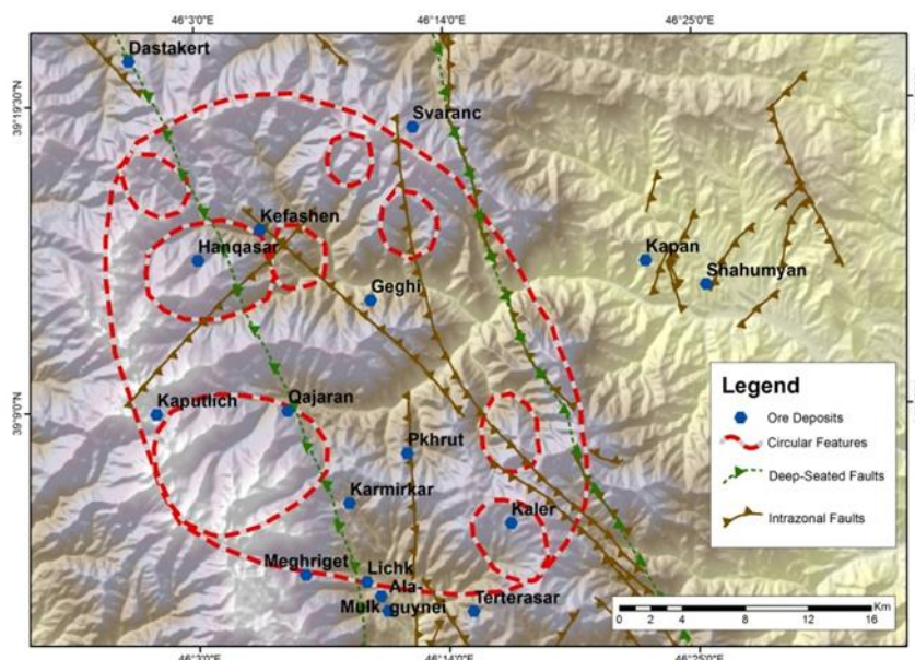
Figure 8. The spatial relationship of ore deposits with the Meghri-Bargushat CS group
